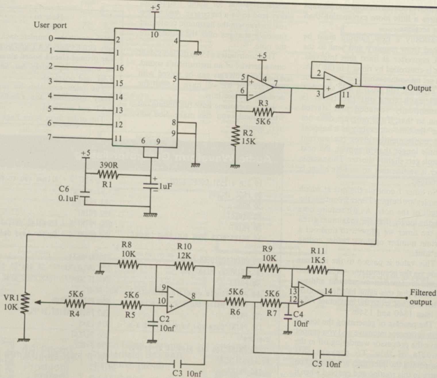
Figure IV: The D/A converter with filtered output
