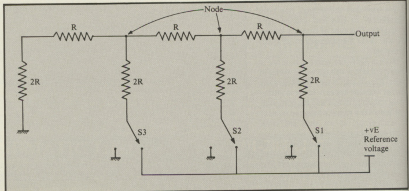
Figure II: A R-2R ladder D/A converter
