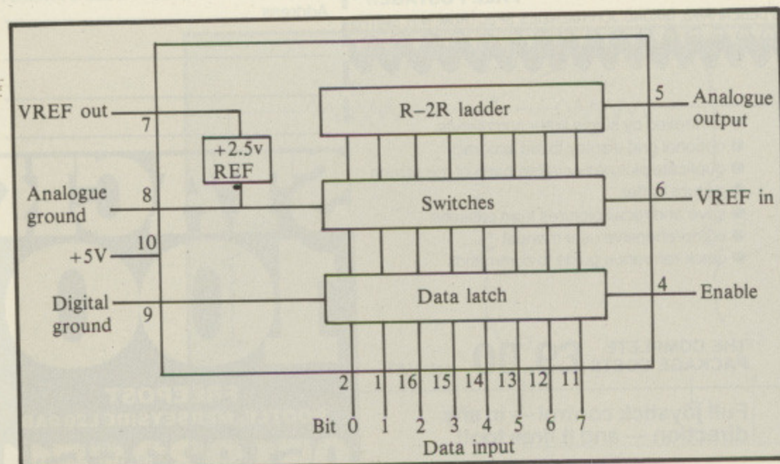
Figure III: Inside the ZN428E-8 D/A converter
