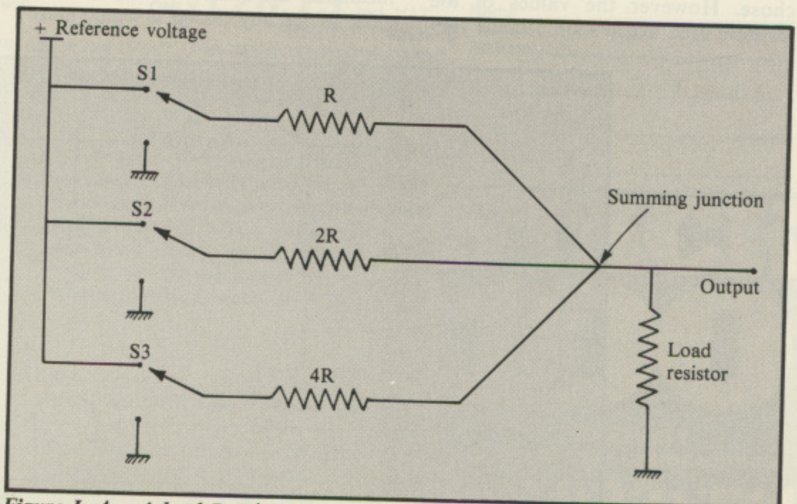
Figure I: A weighted R D/A converter
